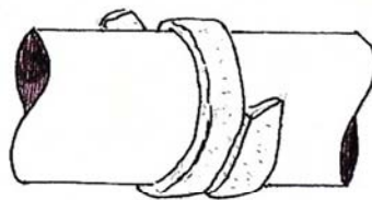
CORRECT (skive joint) (stagger @ 45 degree angle)
