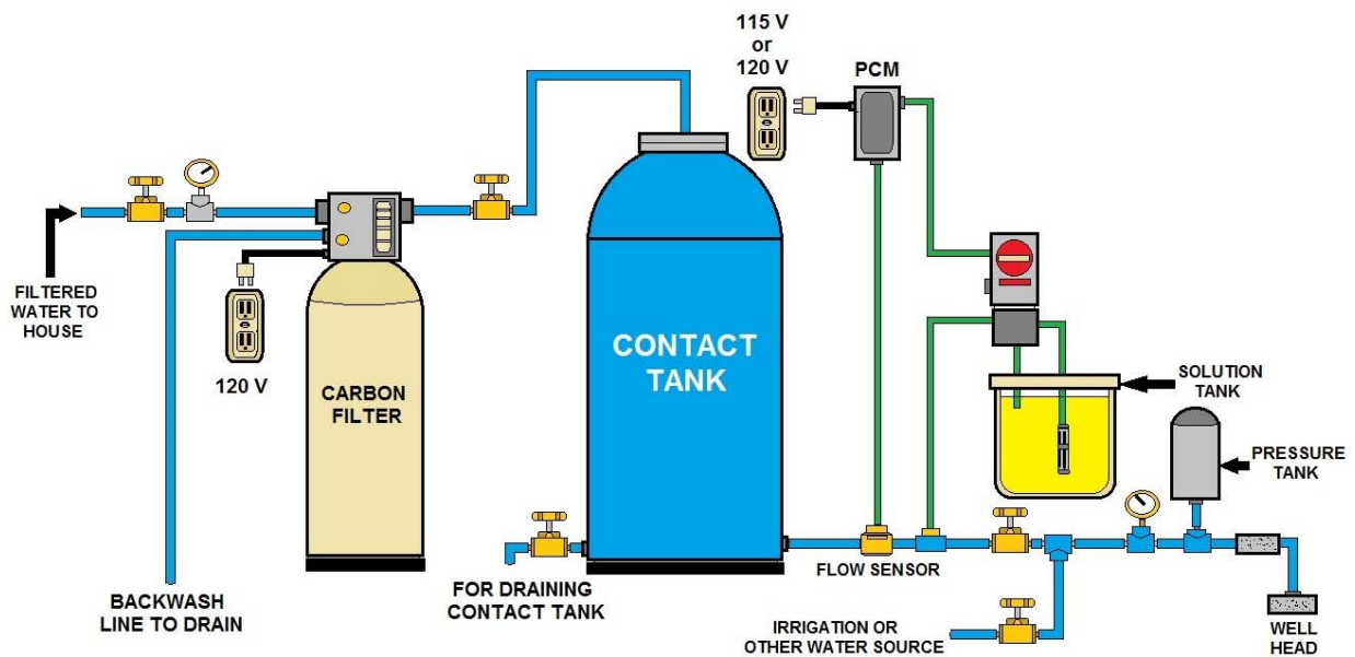
CHLORINATING WELL WATER
