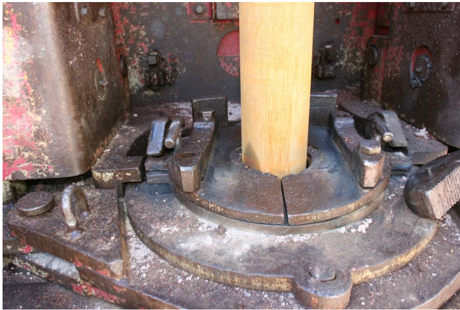
Top, drilling deck, below, well secured under drilling deck with pipe and pipe slip.
