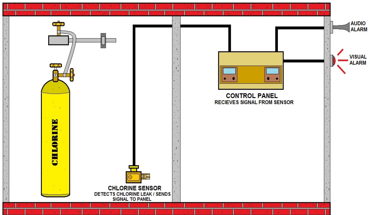
CHLORINE STORAGE ROOM
