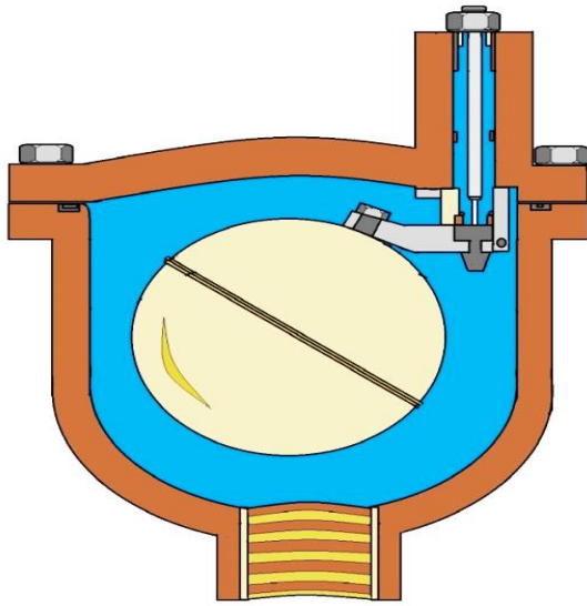
AIR RELIEF VALVE
