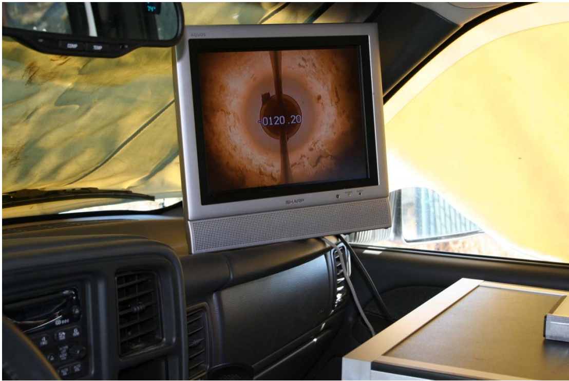
Using a video camera to see inside a groundwater well.
