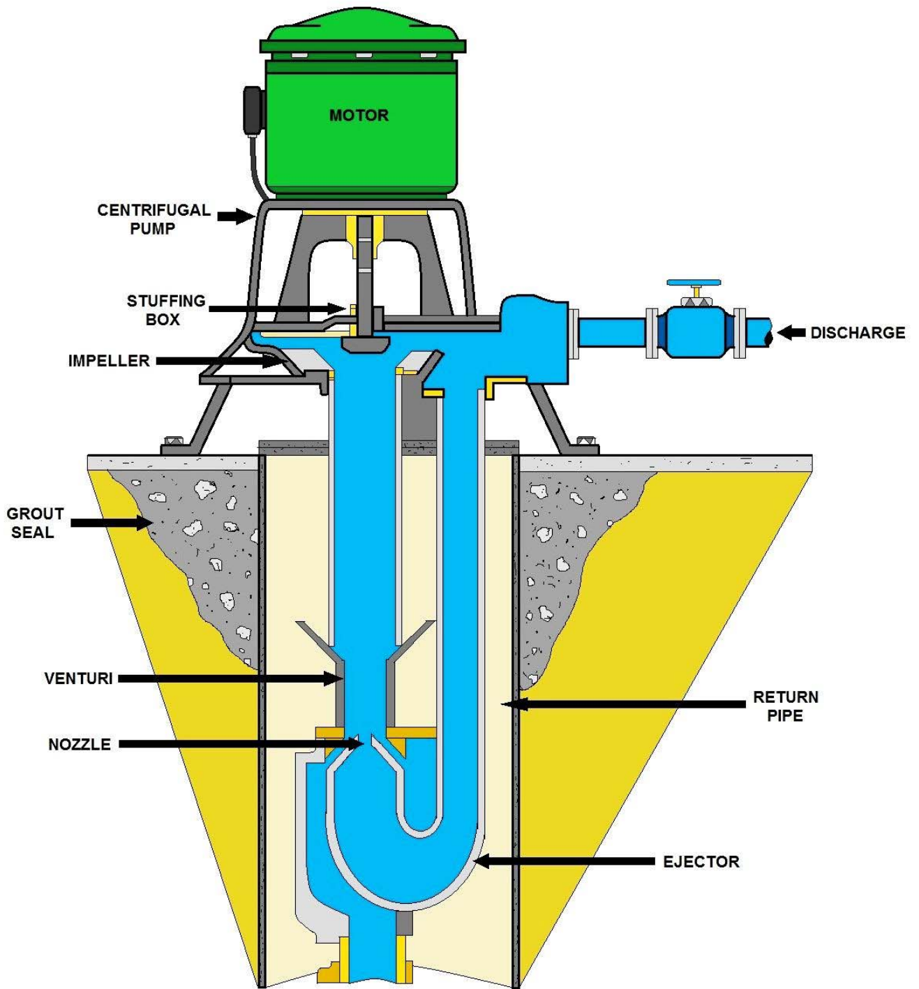
VERTICAL TURBINE INSTALLATION DIAGRAM
