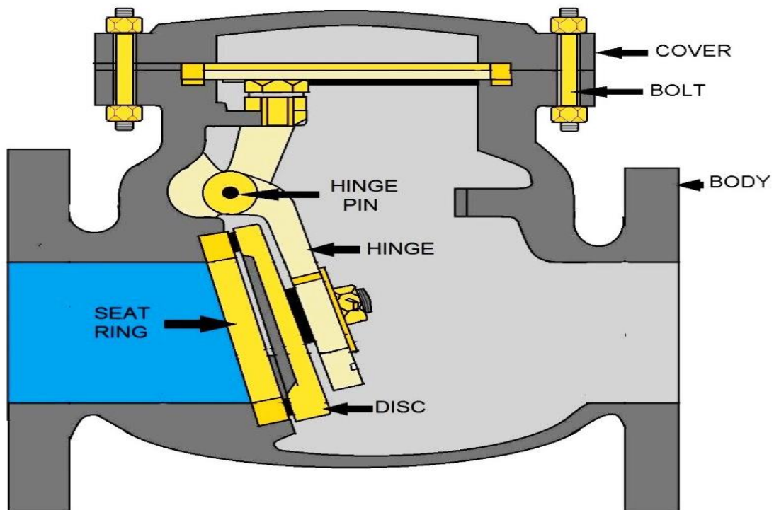
CHECK VALVE
