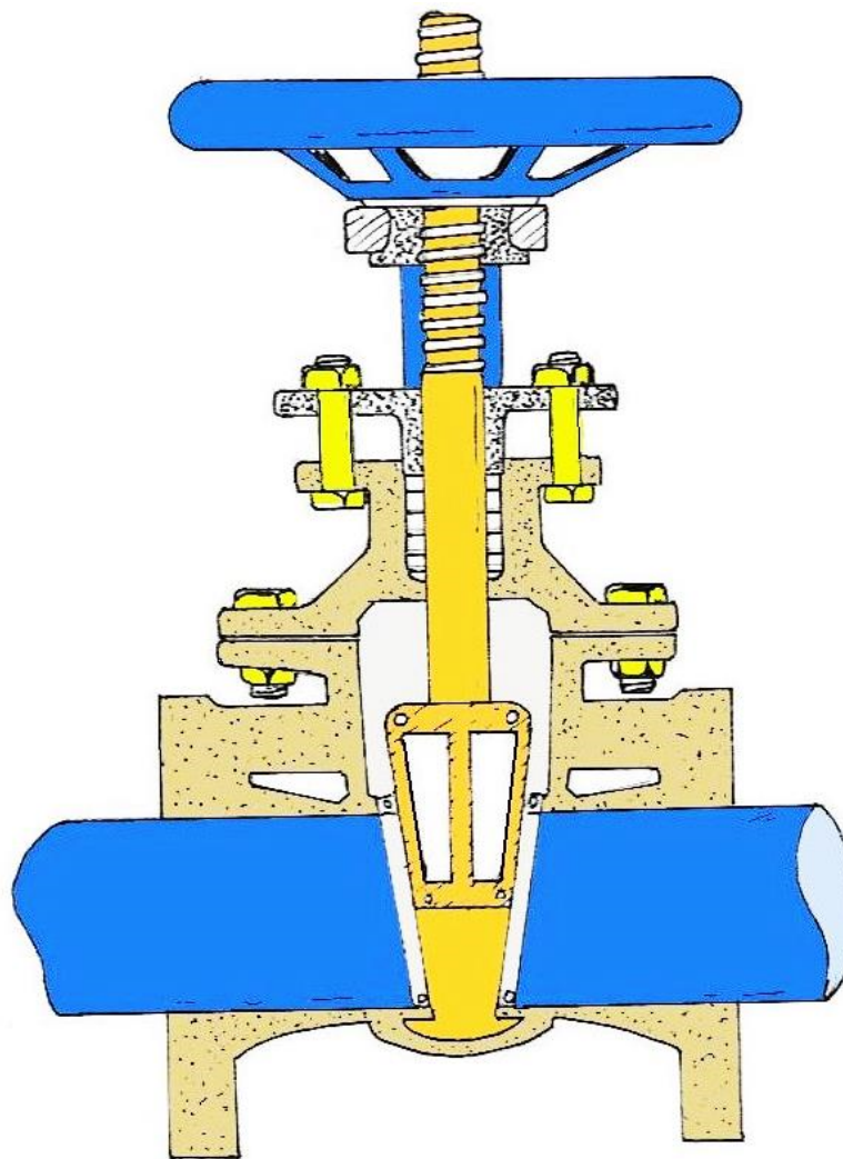
RISING STEM VALVE
