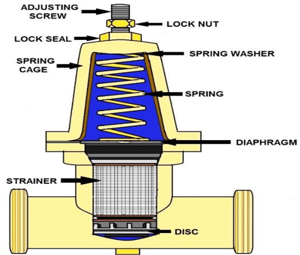
PRESSURE REDUCING VALVE
