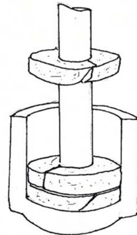
CORRECT (skive joint) (stagger @ 45 degree angle)
