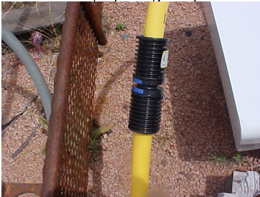
Fusion Butt Joint on plastic pipe Mechanical (compression) joint on plastic
