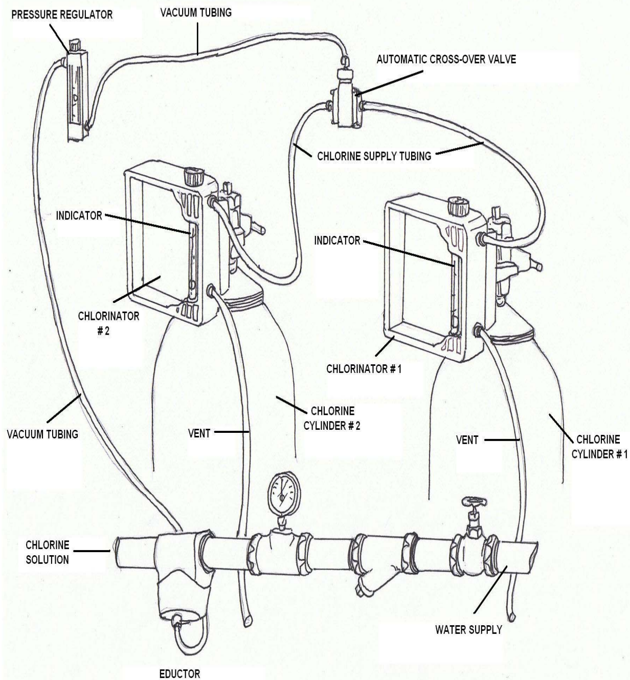
TYPICAL AUTOMATIC CROSS-OVER SYSTEM
