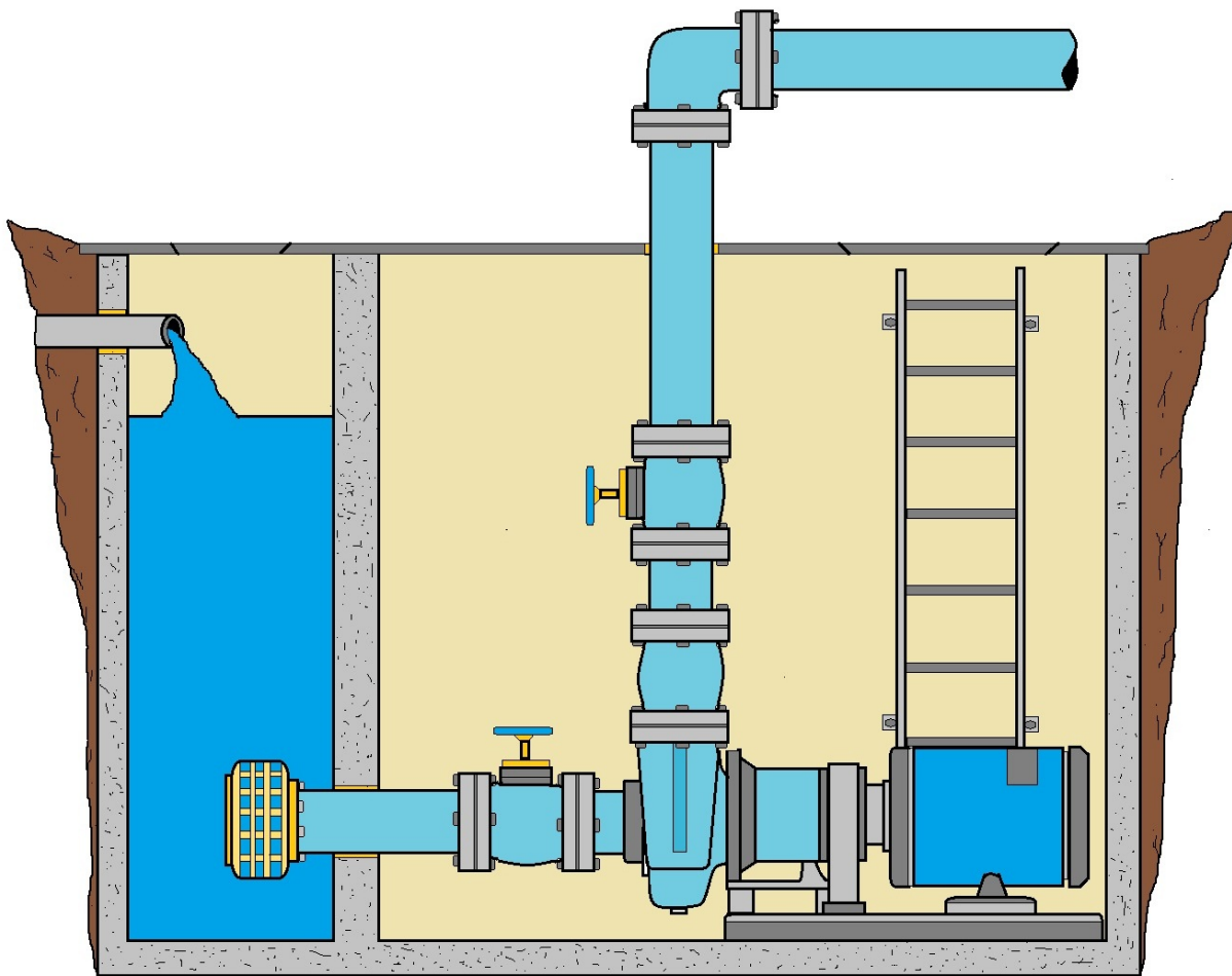
CLOSED COUPLED CENTRIFUGAL PUMP
