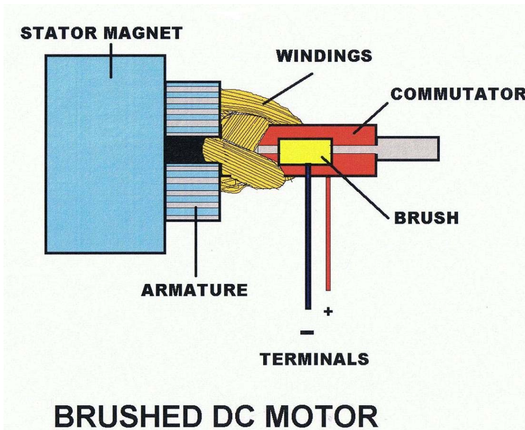
PARTS OF A DC MOTOR
