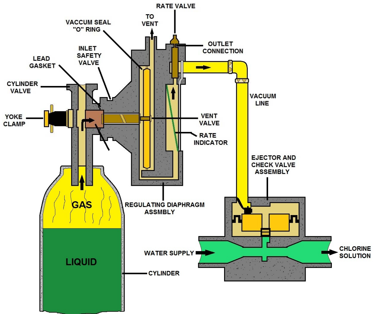
150 Lb. SINGLE CYLINDER CHLORINATOR
