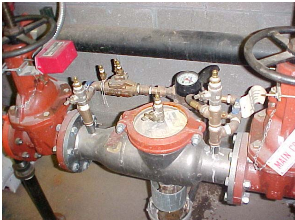
RPDA, Two Reduced Pressure Principle Backflow Assemblies together on a Fireline. Ames SS Assembly. Below an Antifreeze Loop with check valve on a Fireline. Notice the OS&Y Valves (Outside Screw and Yoke).
