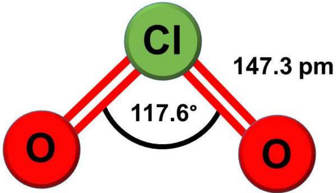
CHLORINE DIOXIDE MOLECULE
