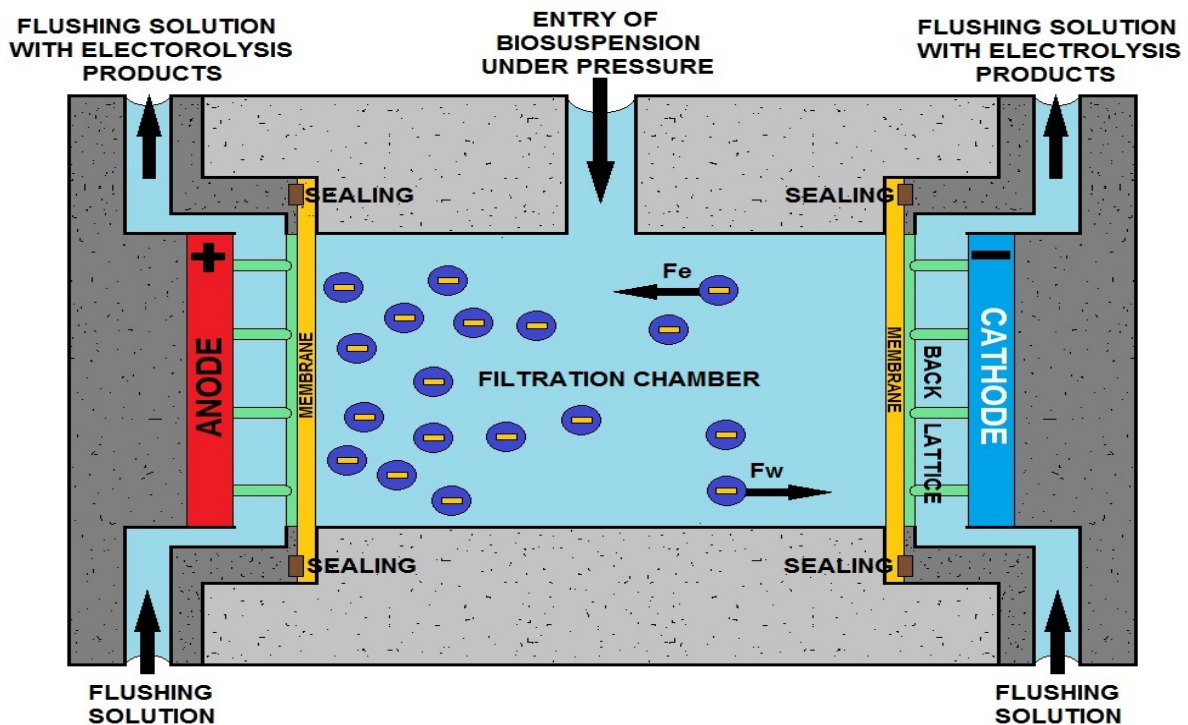
ELECTROFILTRATION CHAMBER
