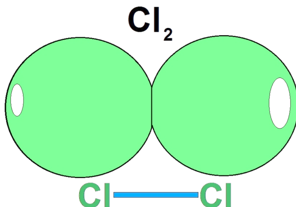
CHLORINE MOLECULAR STRUCTURE
