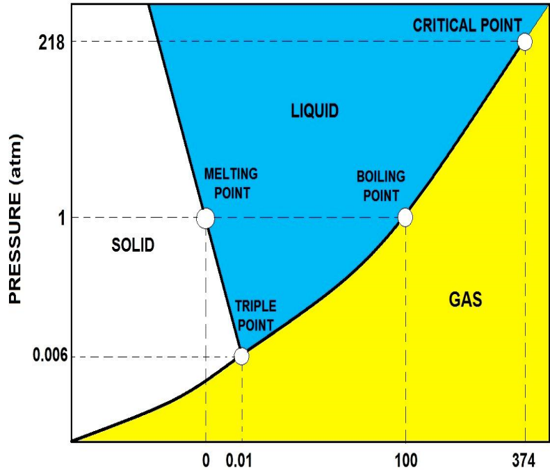
TEMPERATURE (°C) WATER PHASE DIAGRAM
