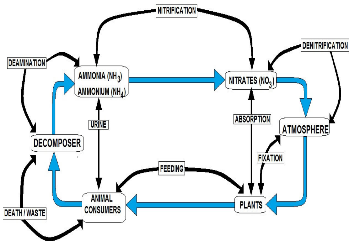
NITROGEN CYCLE
