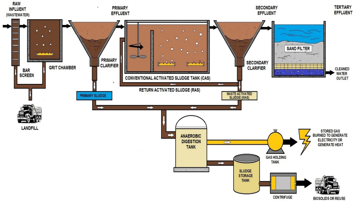
DIAGRAM OF TYPICAL WASTEWATER TREATMENT
