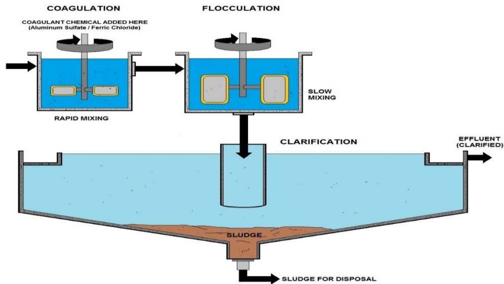
BASIC DIAGRAM OF CHEMICAL COAGULATION PROCESS IN WASTEWATER
