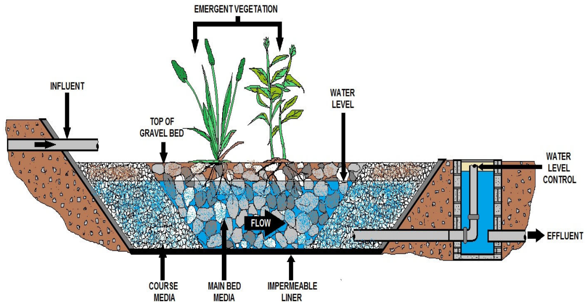
VEGETATIVE SUBMERGED BED (VSB)
