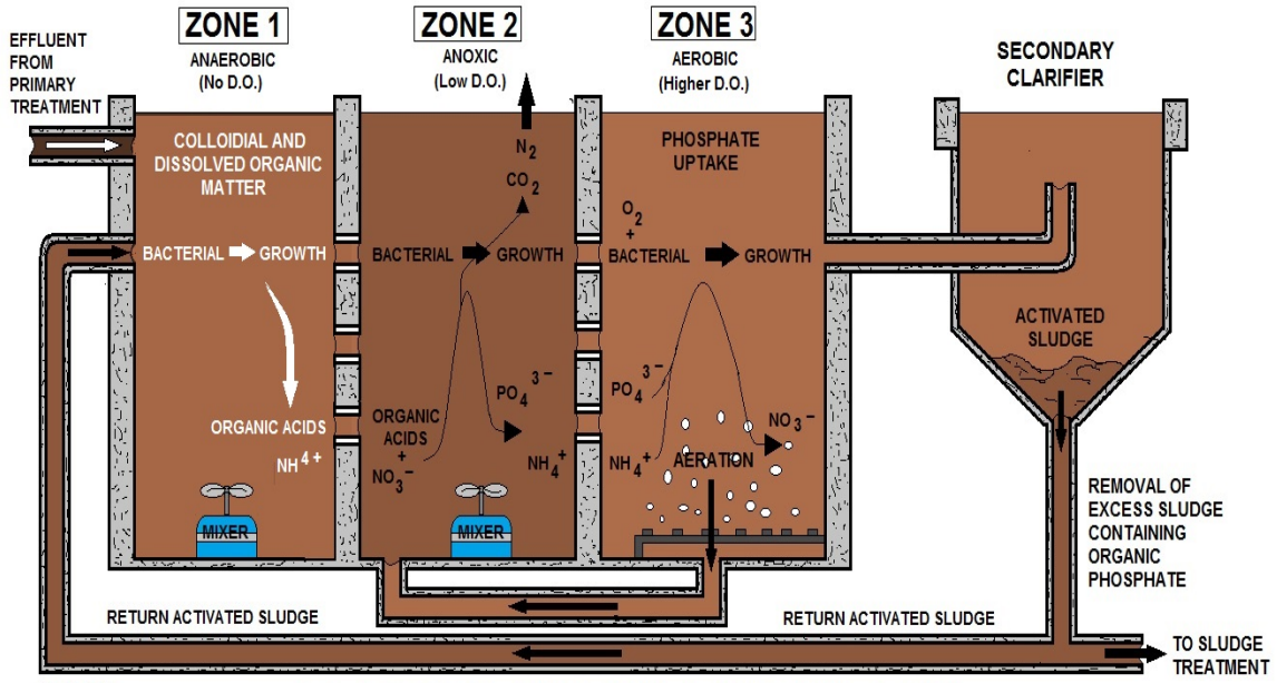
BIOLOGICAL NUTRIENT REMOVAL (BNR)
