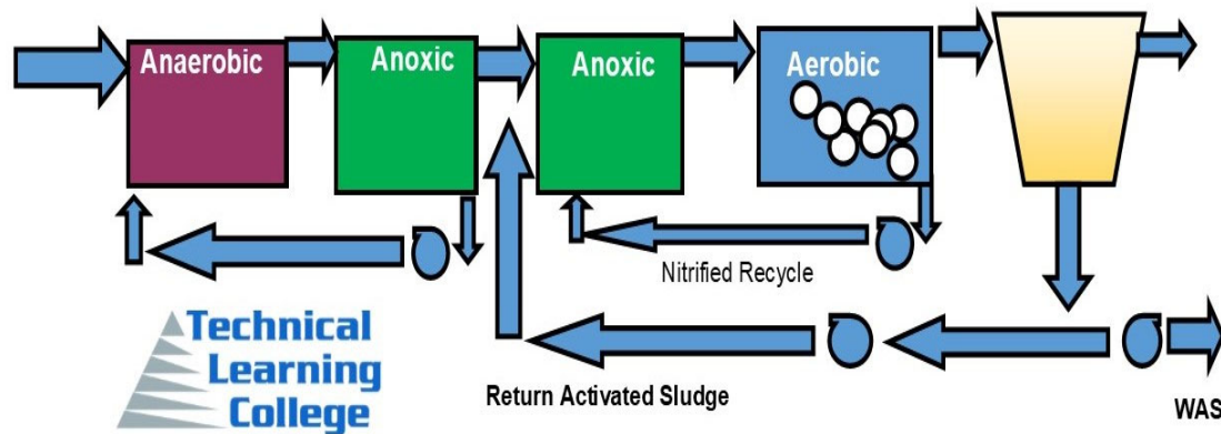
UNIVERSITY OF CAPETOWN (UCT) MODIFIED PROCESS
