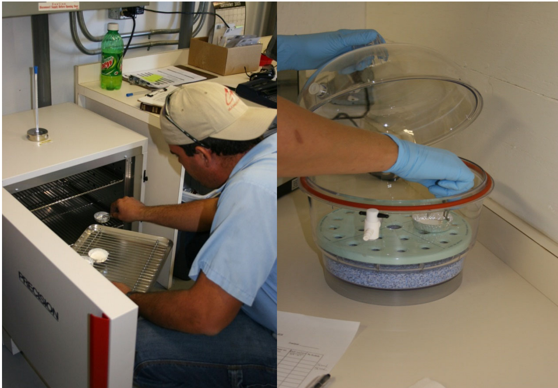
Top left, filters being baked at 105°C. Right photograph, filters in desiccant.
