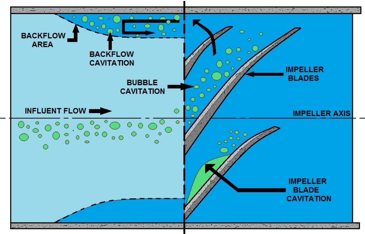
PUMP CAVITATION
