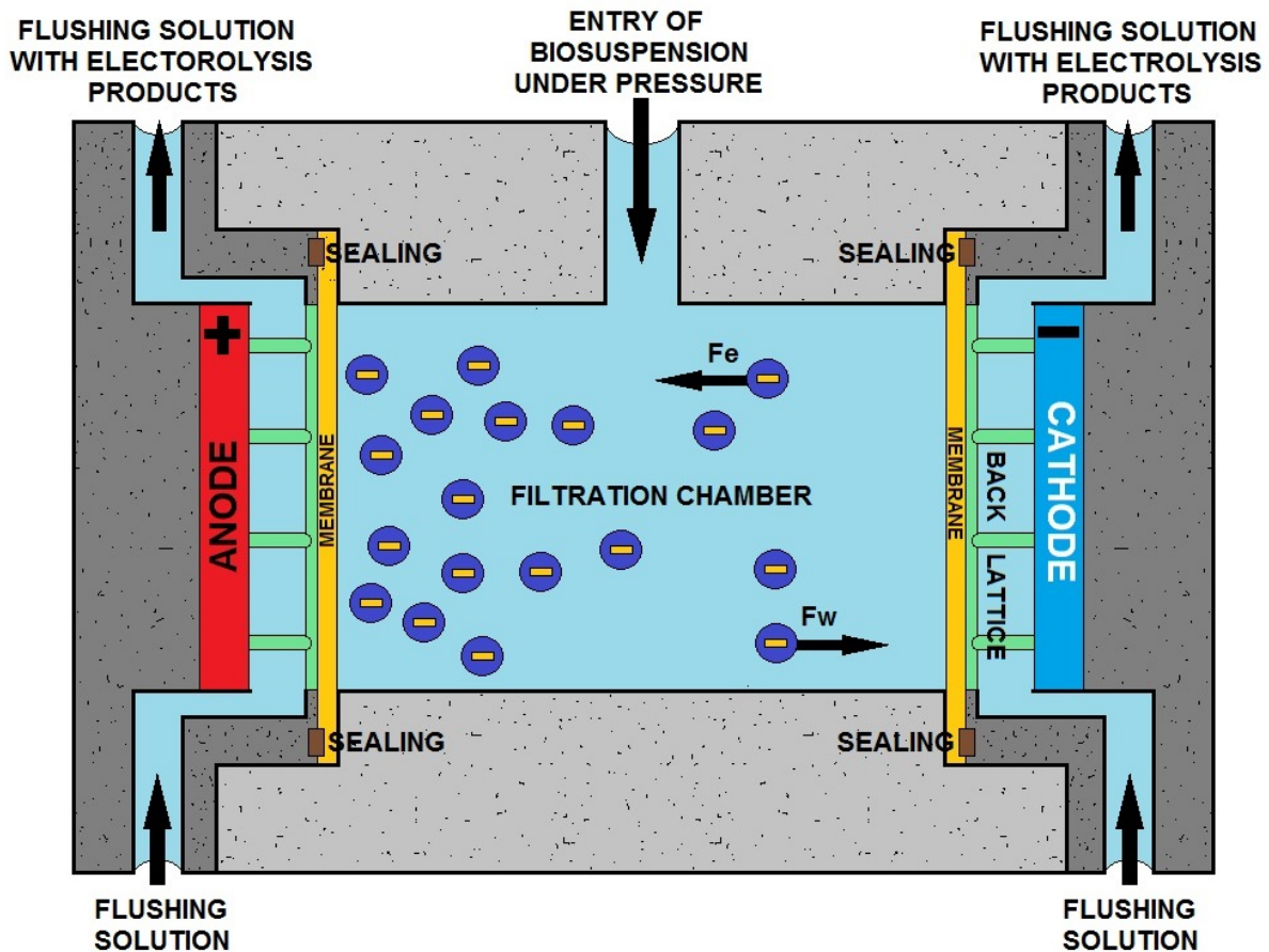
ELECTROFILTRATION CHAMBER
