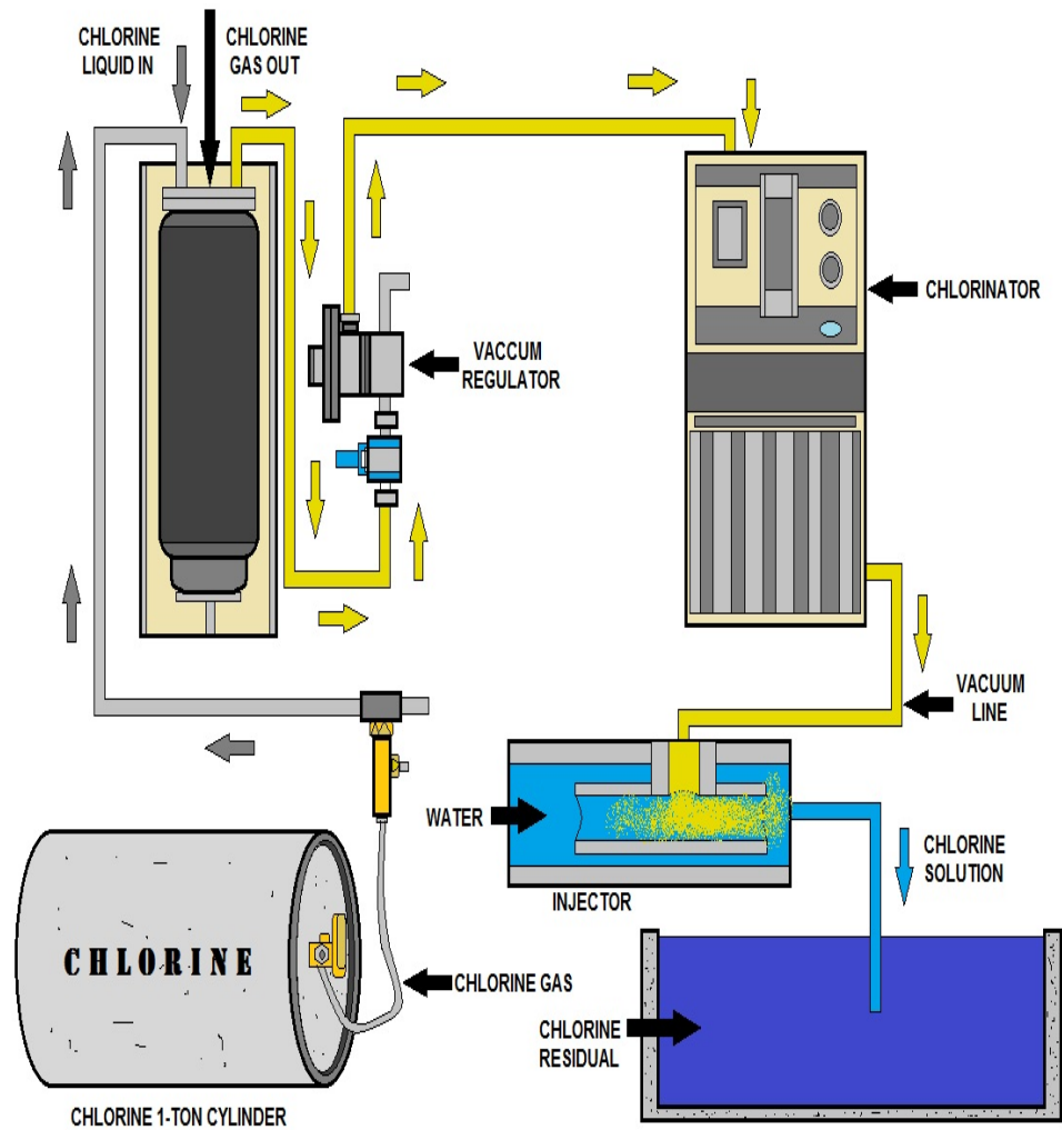
CHLORINE EVAPORATOR – CHLORINATION DIAGRAM
