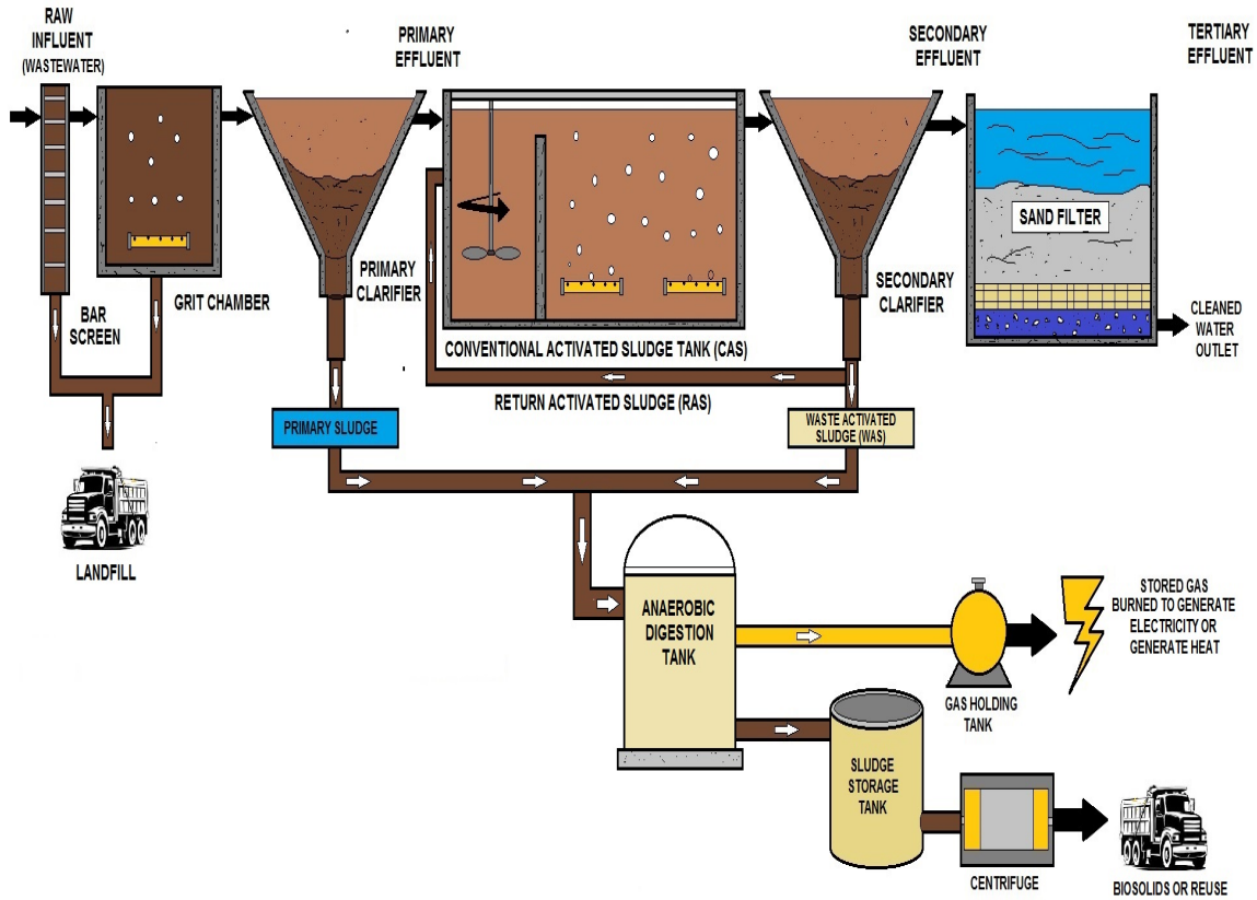
DIAGRAM OF TYPICAL WASTEWATER TREATMENT
