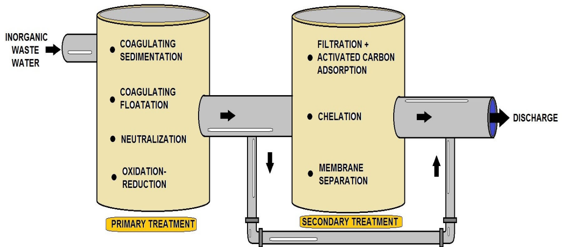
PROCESS OF REMOVING INORGANIC WASTE (Flow Diagram)
