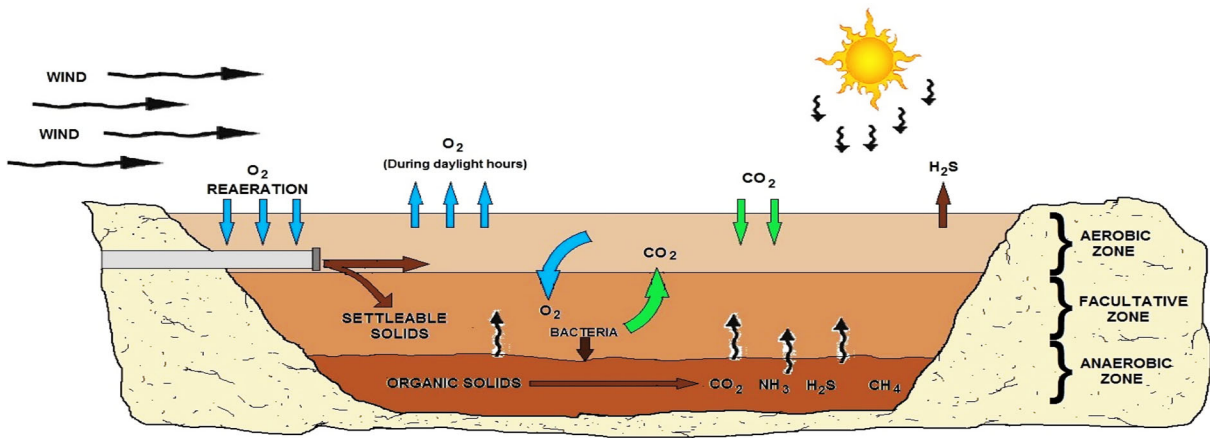
FACULTATIVE LAGOON DIAGRAM
