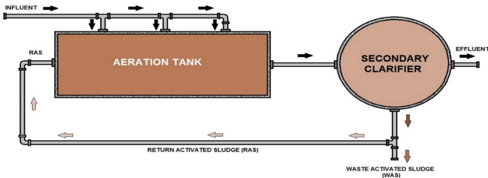
STEP FEED PLANT DIAGRAMS
