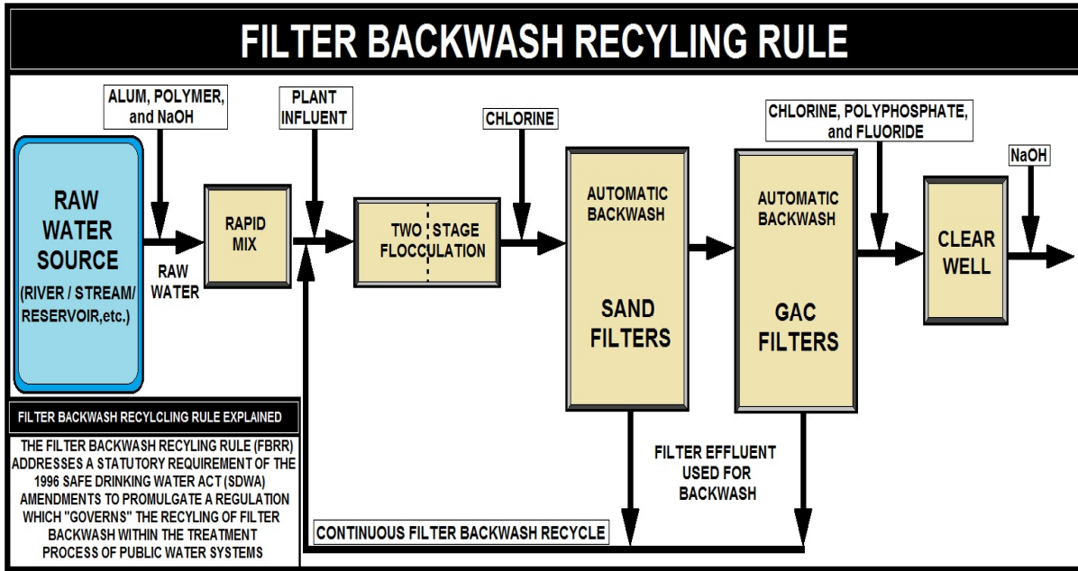
FILTER BACKWASH RECYCLING RULE (FBRR)
