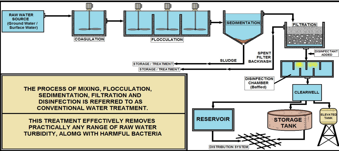
CONVENTIONAL WATER TREATMENT OVERVIEW
