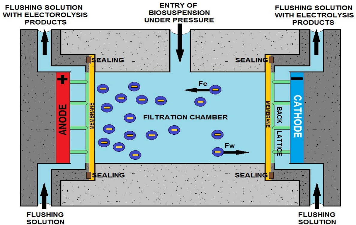
ELECTROFILTRATION CHAMBER
