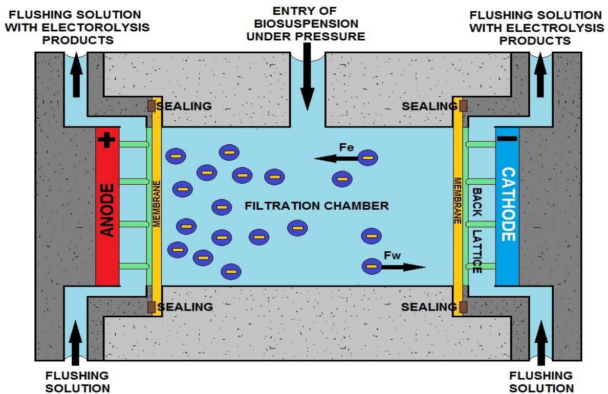
ELECTROFILTRATION CHAMBER
