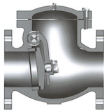
Plain Swing check valve
