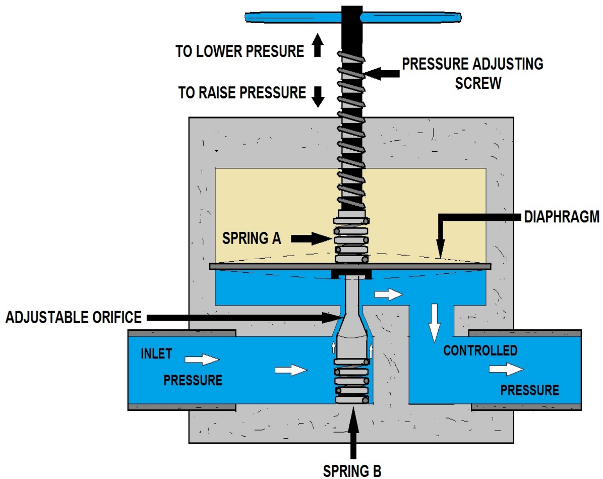
PRESSURE-REGULATING VALVE
