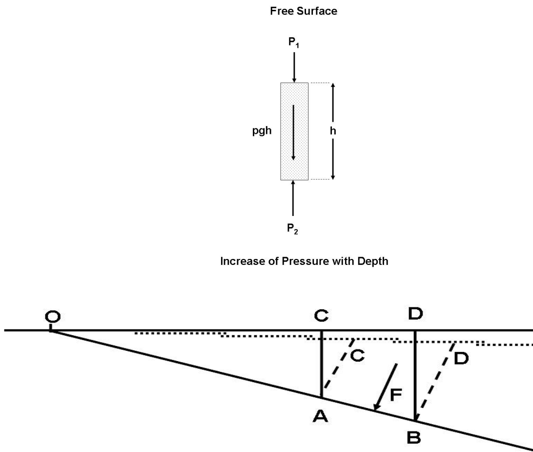
THRUST ON A PLANE DIAGRAM
