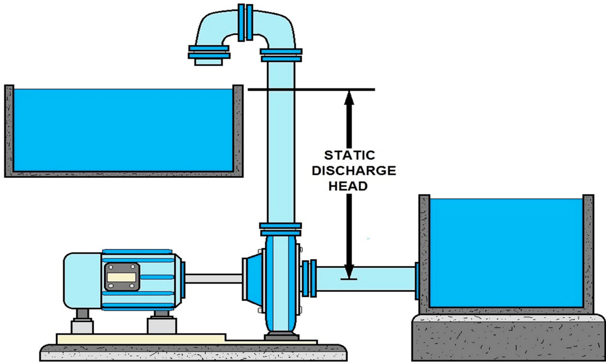
EXAMPLE OF STATIC DISCHARGE HEAD (The vertical distance from discharge outlet to point of discharge)
