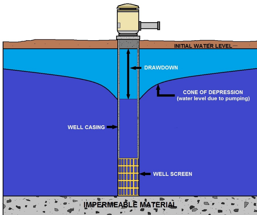
CONE OF DEPRESSION CAUSED BY PUMPING
