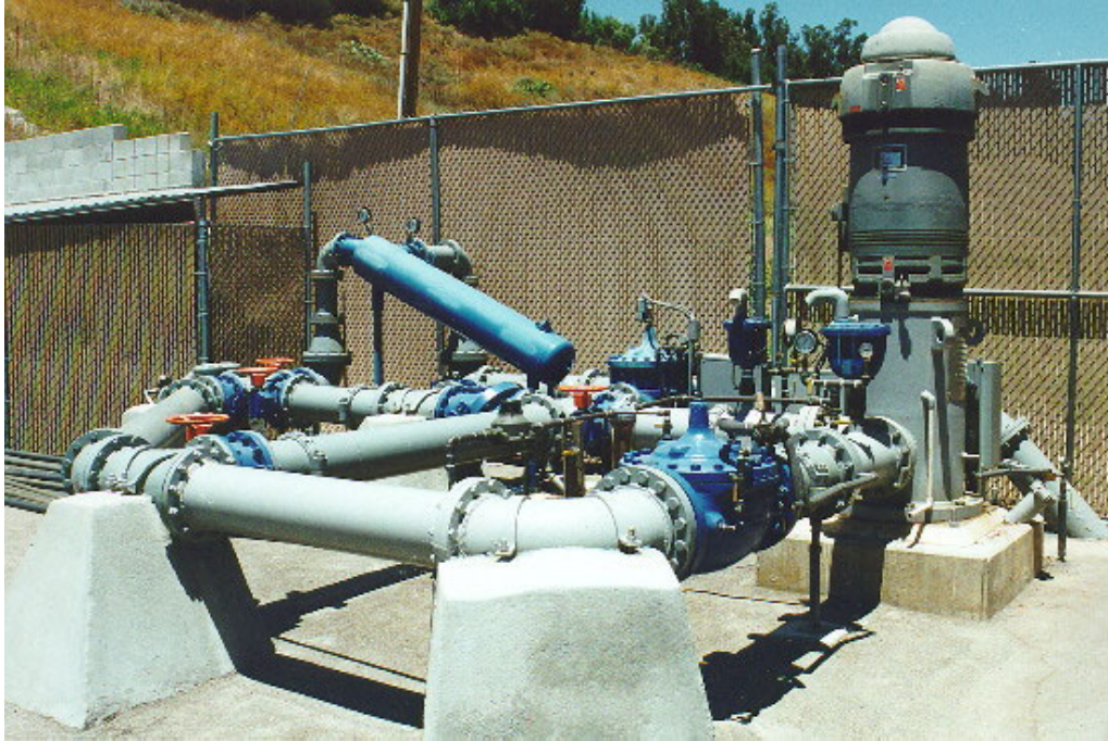
Vertical Turbine Well
