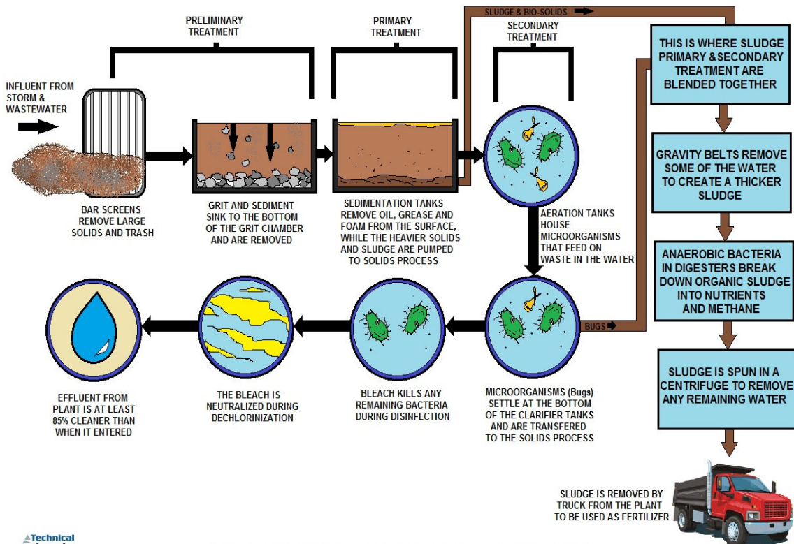
USING MICROORGANISMS TO CLEAN WASTEWATER
