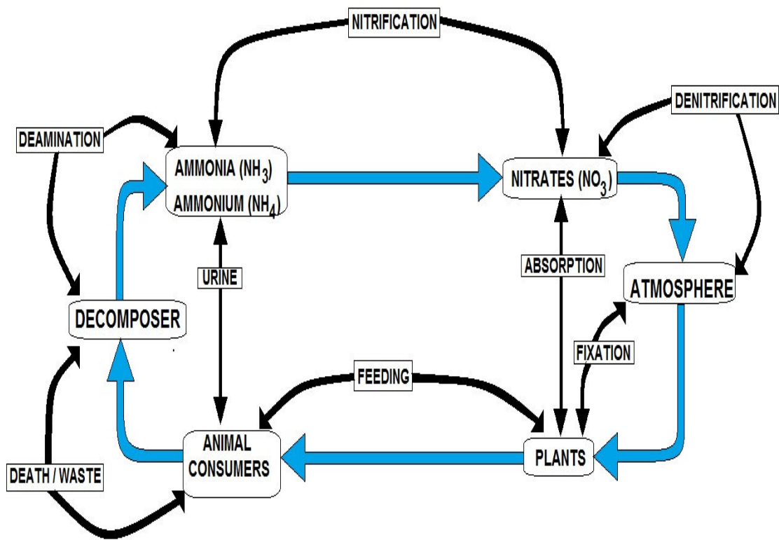
NITROGEN CYCLE
