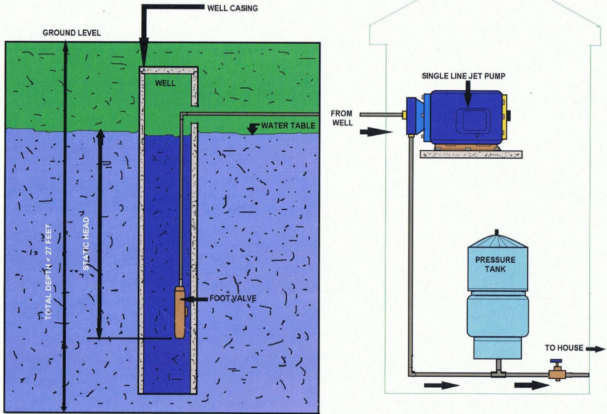
SHALLOW WELL WITH SINGLE-LINE JET PUMP (SUITABLE FOR SHALLOW WELLS LESS THAN 27 FEET DEEP)
