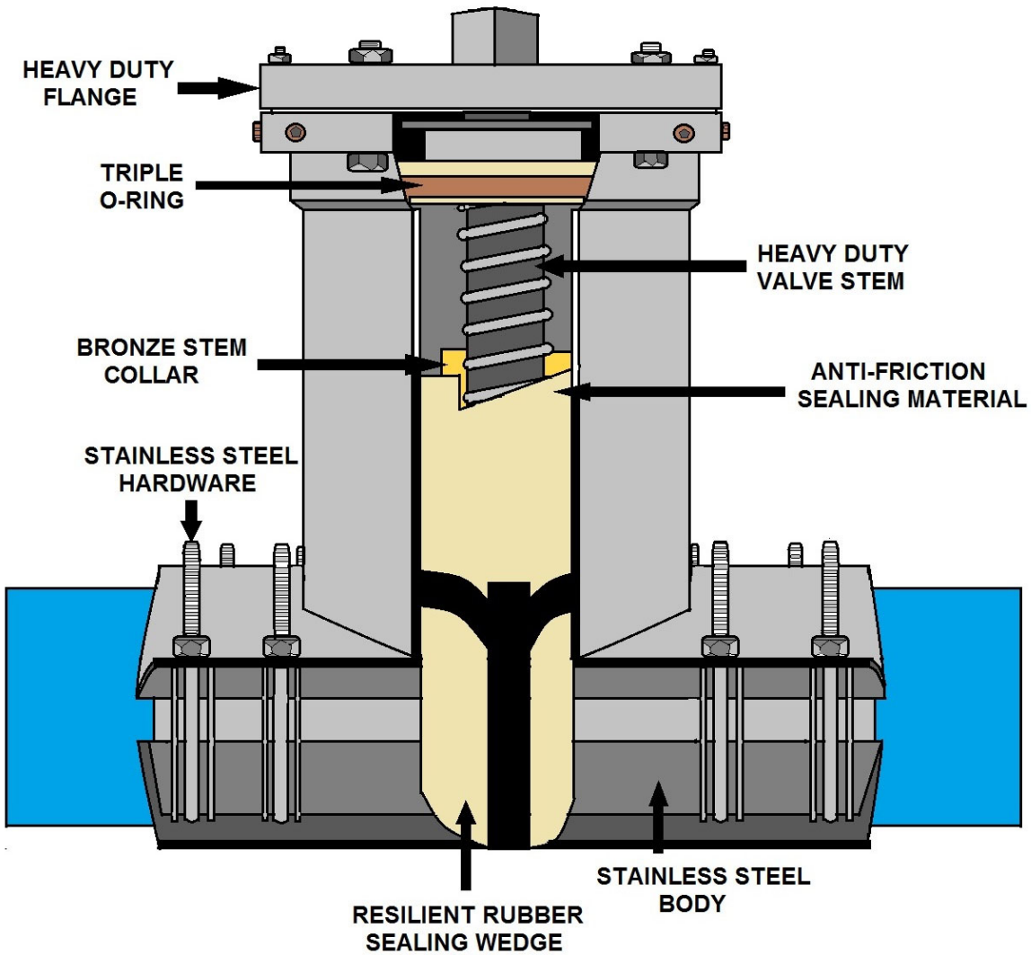
INSTA-VALVE DIAGRAM
