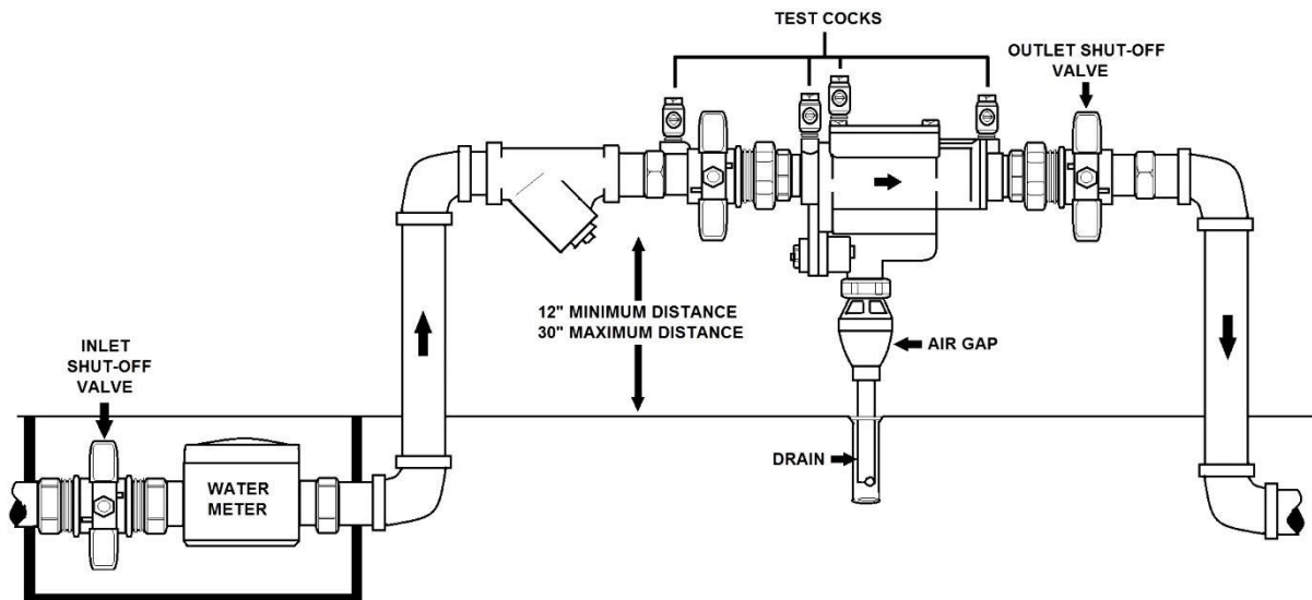
REDUCED PRESSURE BACKFLOW PREVENTER
