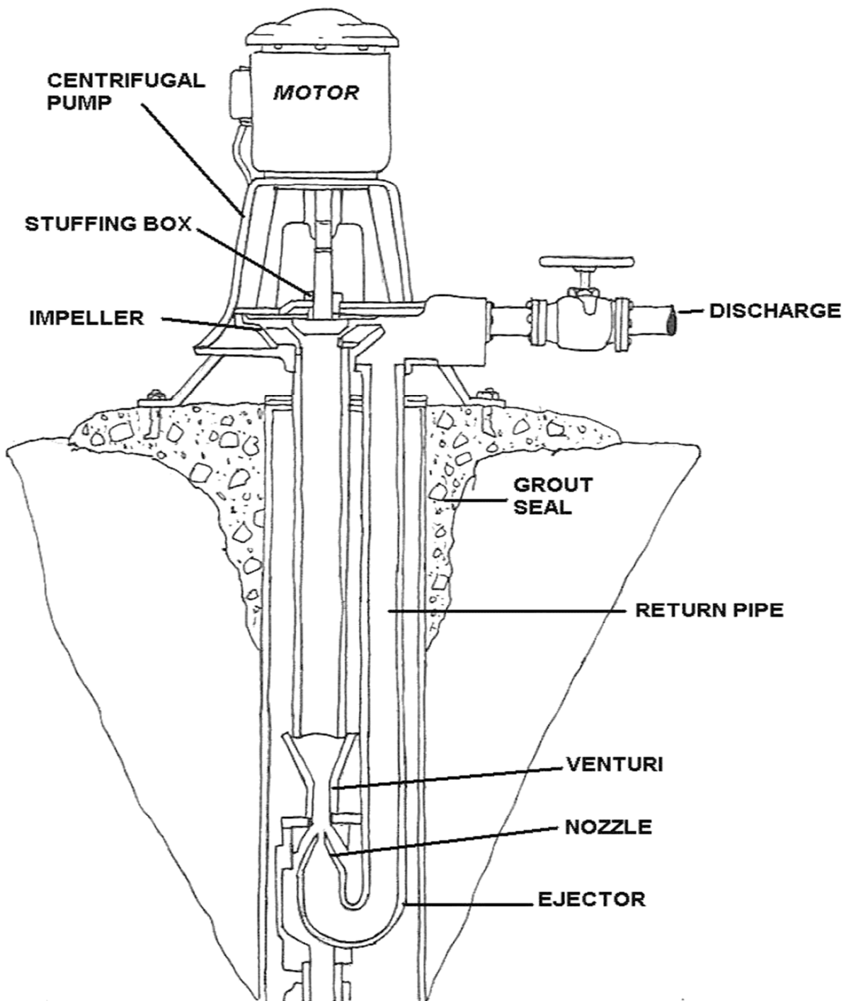
VERTICAL TURBINE PUMP DIAGRAM #2
