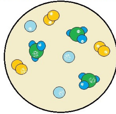
MIXTURE OF TWO ELEMENTS AND A COMPOUND
