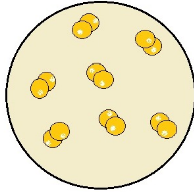
MOLECULES OF AN ELEMENT
