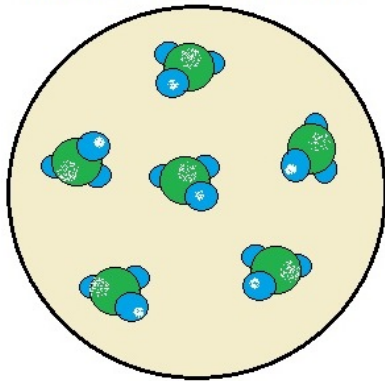
MOLECULES OF A COMPOUND
