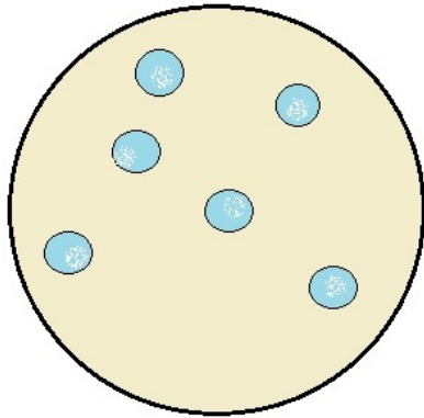
ATOMS OF AN ELEMENT
