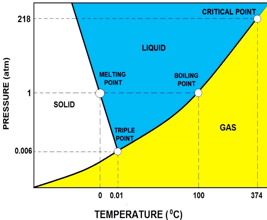
WATER PHASE DIAGRAM
