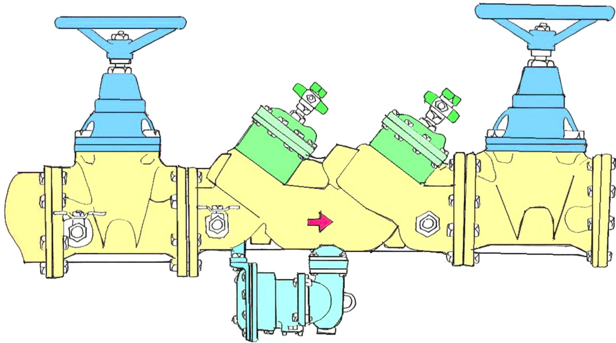
REDUCED PRESSURE PRINCIPLE BACKFLOW ASSEMBLY
