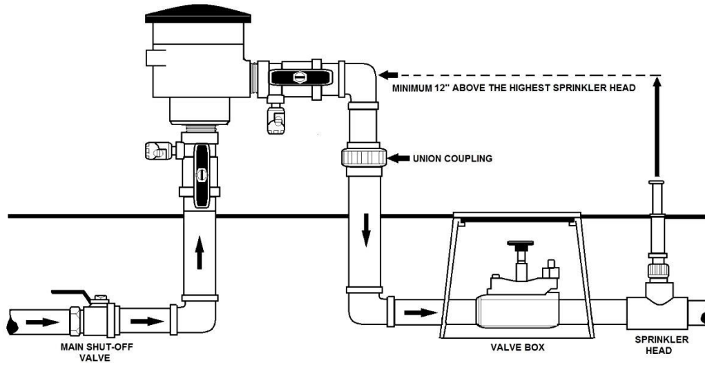
PRESSURE VACUUM BREAKER BACKFLOW PREVENTER
