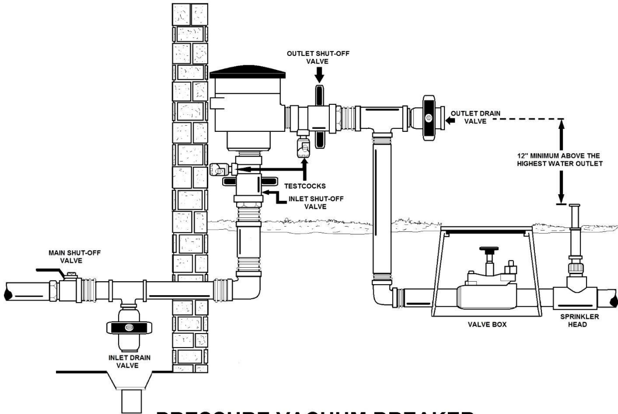
PRESSURE VACUUM BREAKER
