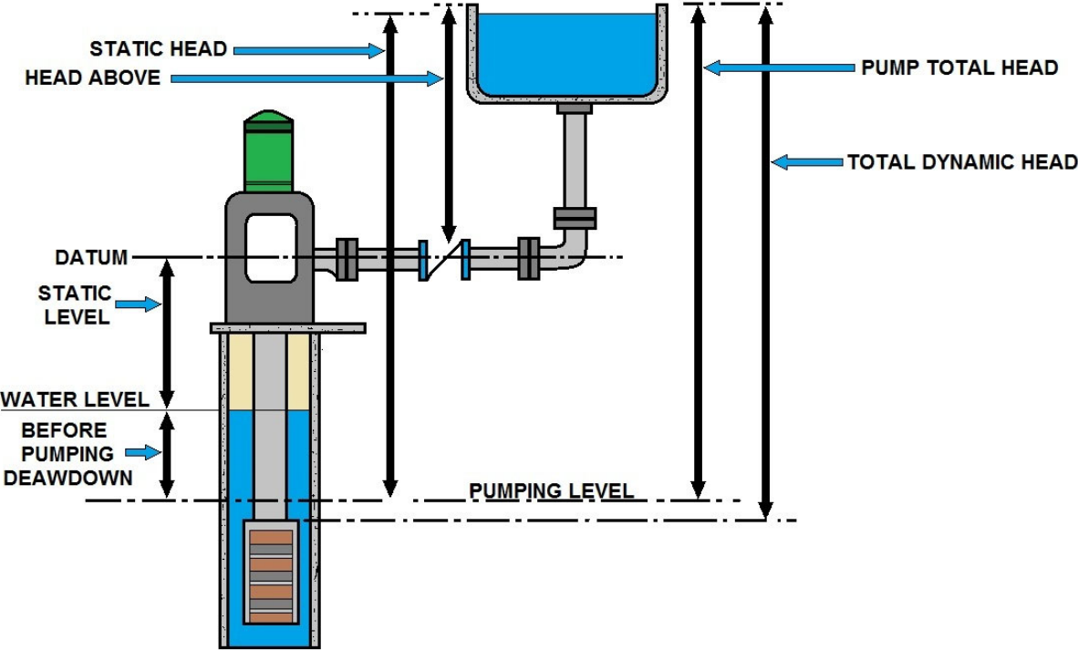
PUMPING HEAD DIAGRAM #1
