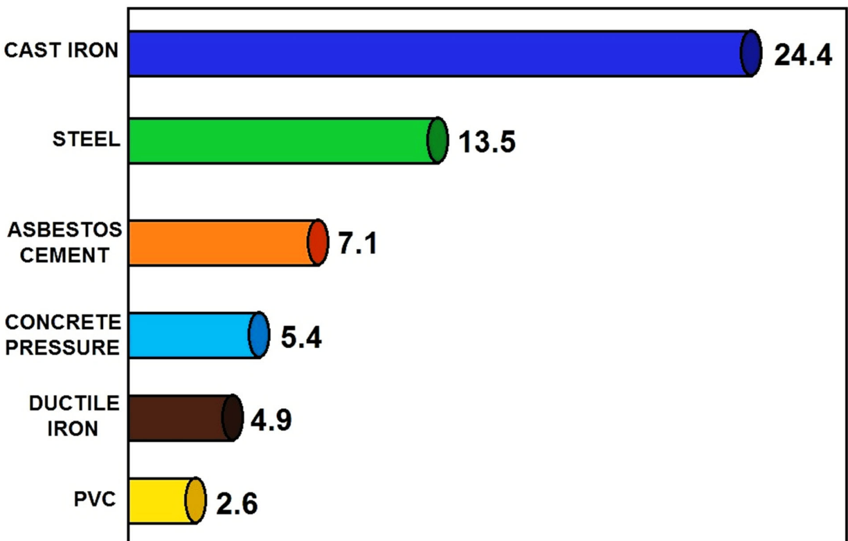
WATER MAIN BREAKS RATES REFLECT # OF BREAKS PER 100 MILES OF INSTALLED PIPE
