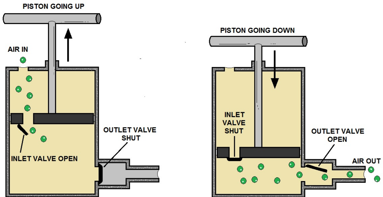
BICYCLE PUMP BASIC OPERATION
