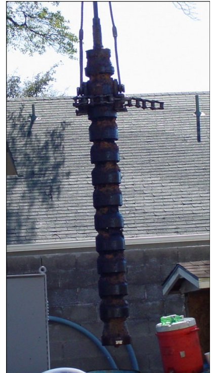
Above, Vertical Turbine Pump Being Removed (notice line shaft)
