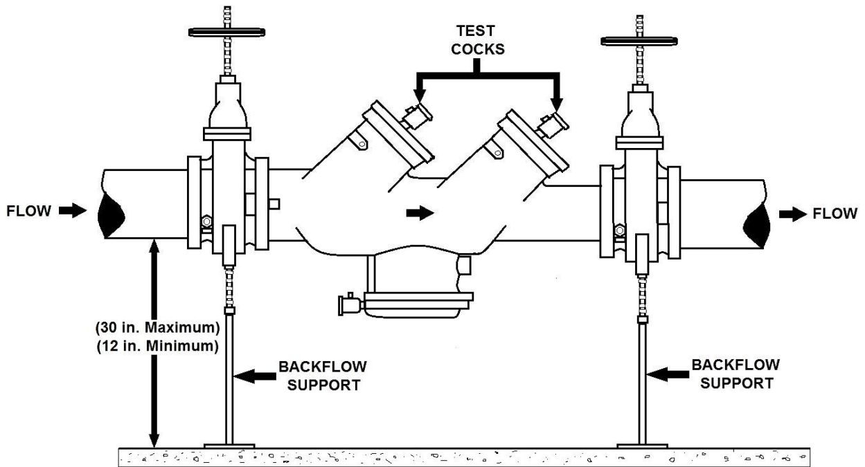
DOUBLE CHECK VALVE
