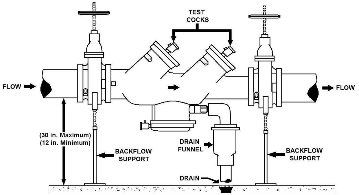
REDUCED PRESSURE BACKFLOW PREVENTER (Indoor Installation)
