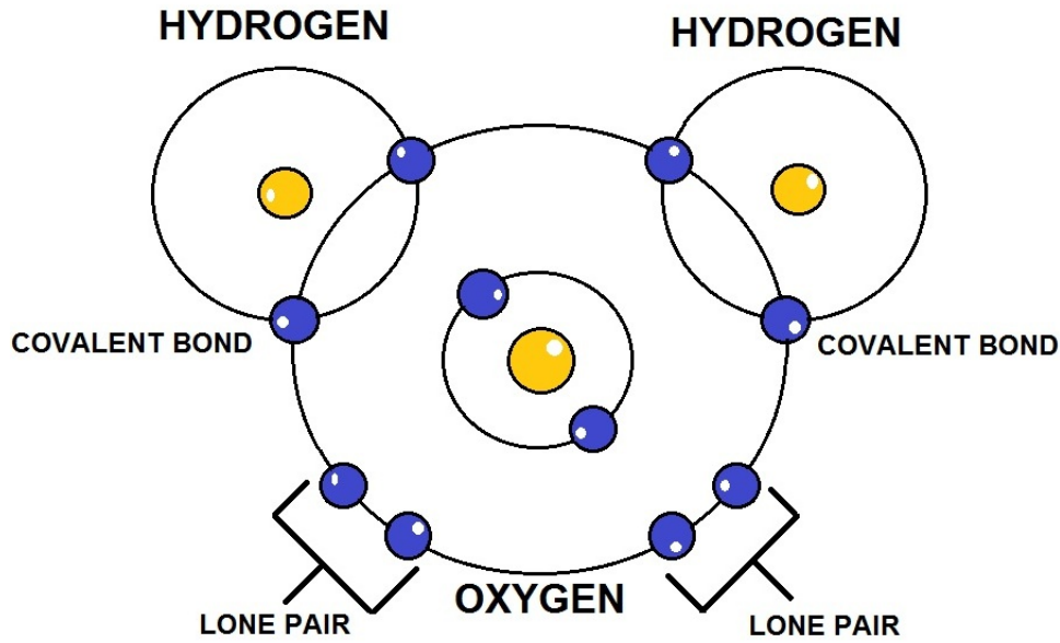
WATER MOLECULE DIAGRAM
