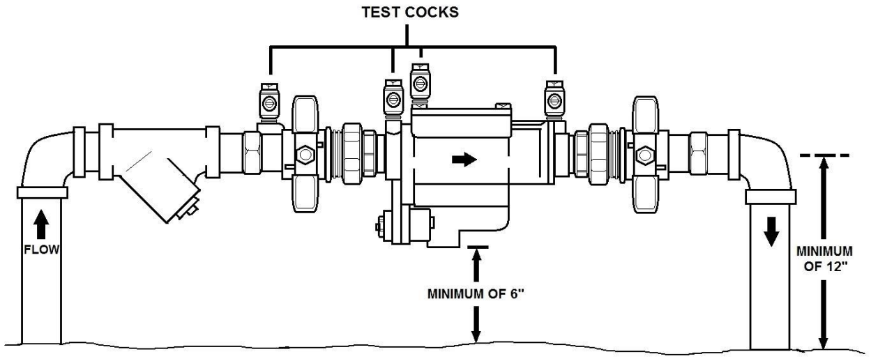
REDUCED PRESSURE BACKFLOW PREVENTER
