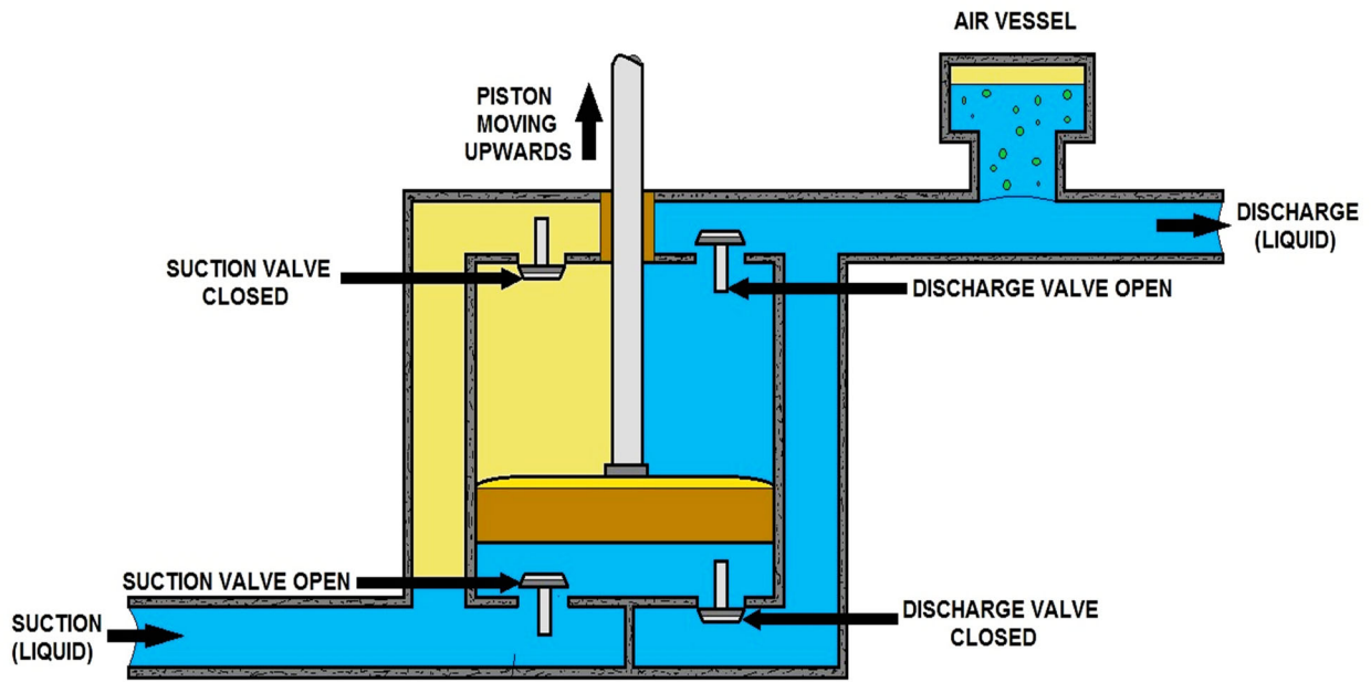
POSITIVE DISPLACEMENT PUMP RECIPROCATING PISTON TYPE
