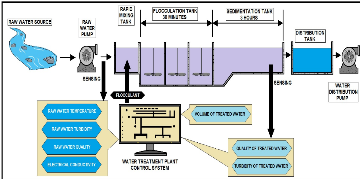
RAW WATER TURBIDITY MONITORING
