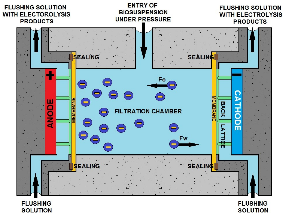
ELECTROFILTRATION CHAMBER
