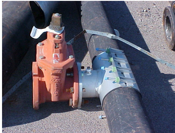
Tapping Sleeve
