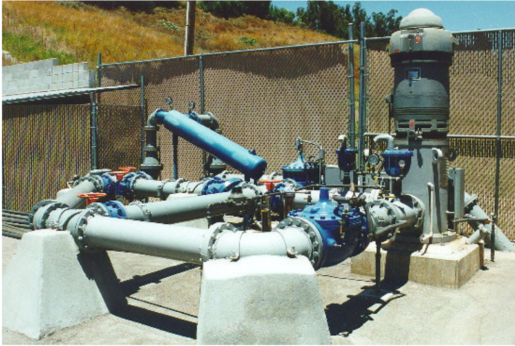
VERTICAL TURBINE WELL EXAMPLE
