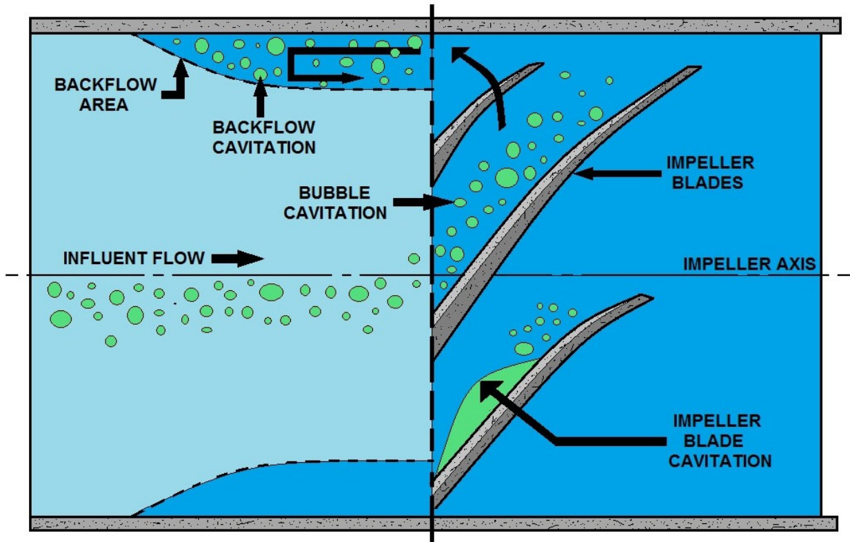
PUMP CAVITATION
