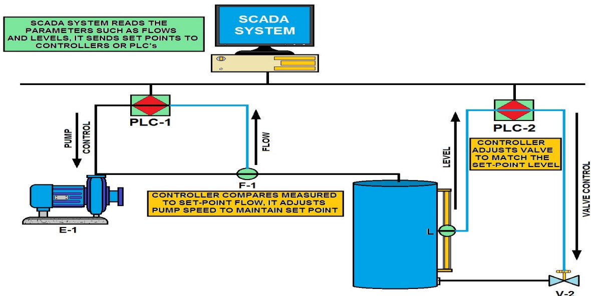
SCADA SYSTEM (SUPERVISORY CONTROL and DATA ACQUISITION)
