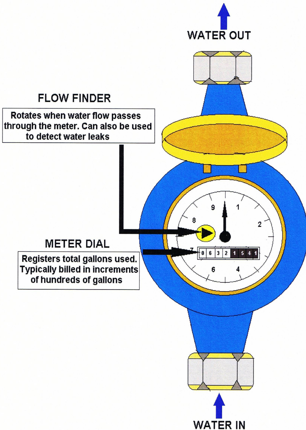
RESIDENTIAL WATER METER (5/8 OR 3/4")
