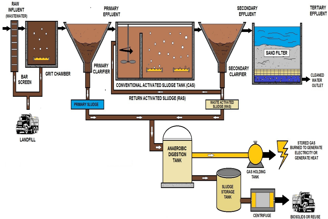
DIAGRAM OF TYPICAL WASTEWATER TREATMENT
