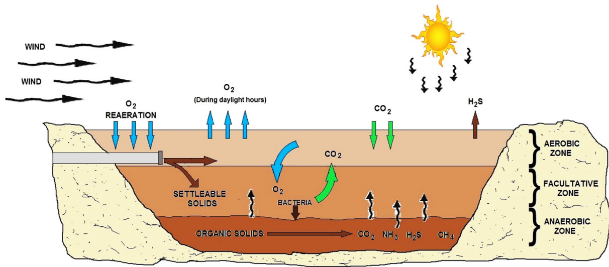
FACULTATIVE LAGOON DIAGRAM
