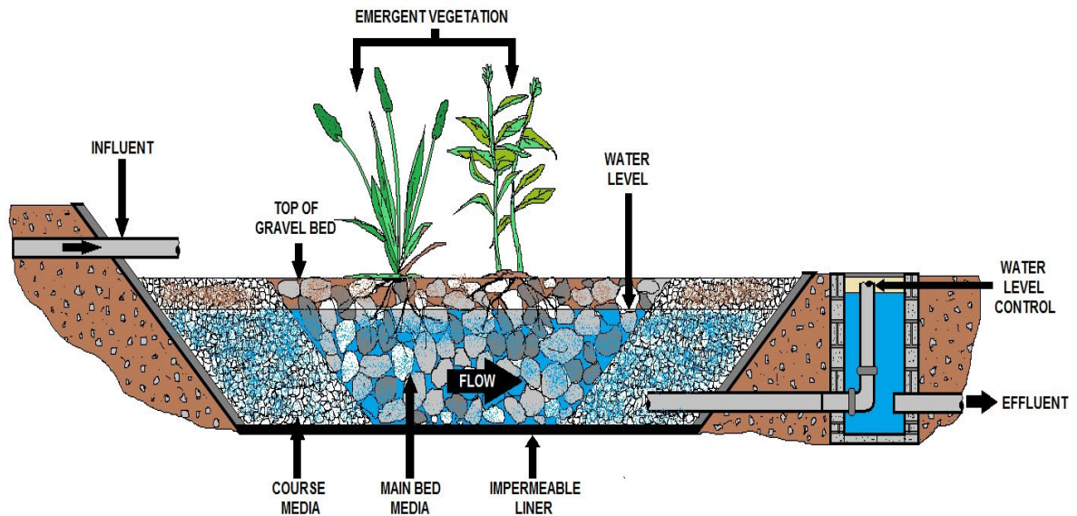
VEGETATIVE SUBMERGED BED (VSB)
